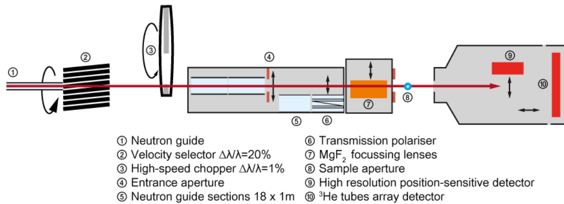
Figure 2: Schematic drawing of KWS-2.
