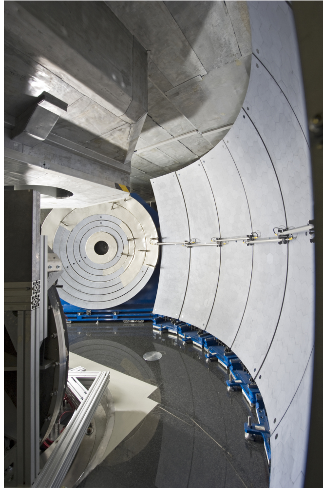
Figure 1: View inside SPHERES: the large array of Si(111) analyzer crystals covers a solid angle of about 2.5, which is 20 % of 4\pi (Copyright by A. Heddergott, TUM).
